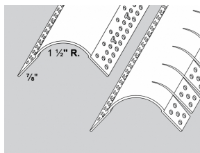
BULLNOSE BEADS 1 1/2" R. Bullnose Outside Corner Bead & Archway
