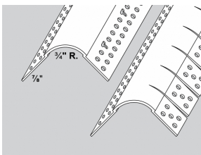
BULLNOSE BEADS 3/4" R. Bullnose Corner Bead & Archway
