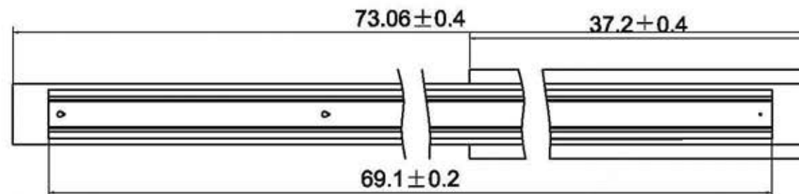
Header and Track Assembly Material: Aluminium+Wood Finish: Aluminium Q.TY: 1pc
