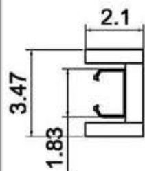
Header and Track Assembly Material: Aluminium+Wood Finish: Aluminium Q.TY: 1pc
