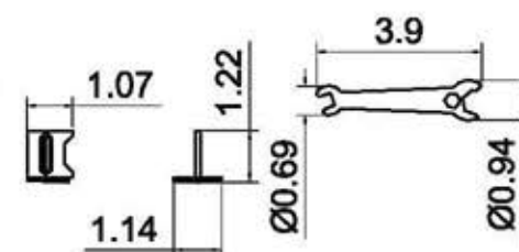
Wrench Material: Steel Thickness: 0.078" Finish: Zinc Q.TY: 1pc
